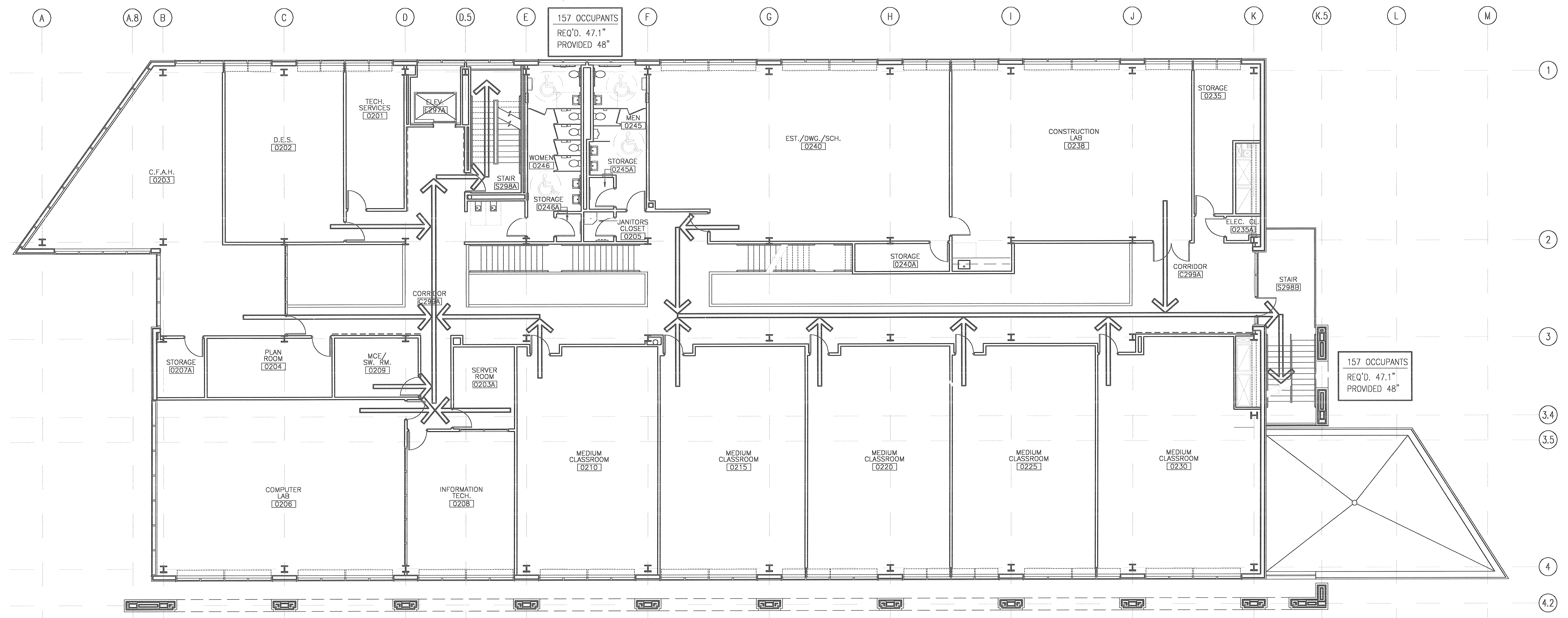
2 SECOND LEVEL EGRESS PLAN 1/8" = 1'-0"
